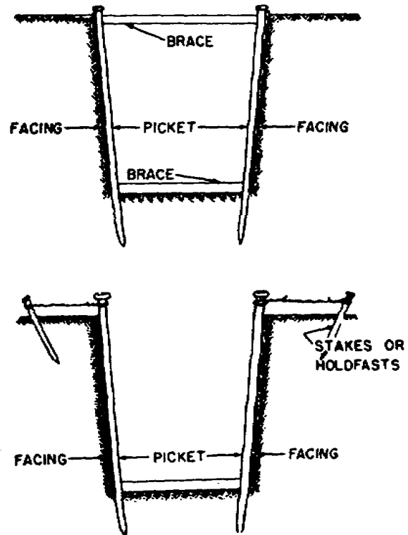
Figure 2-16. Facing revetment supported by pickets.
